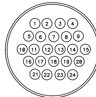
END VIEW OF RECEPTACLE
