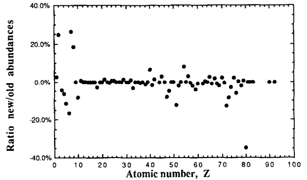
FIG. 1. Comparison of new solar-system abundances with those of ANDERS and EBIHARA (1982).
