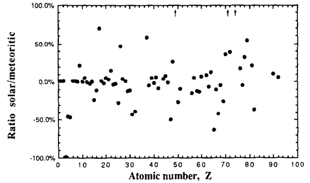
FIG. 2. Comparison of solar-system ("meteoritic") and photospheric abundances.
