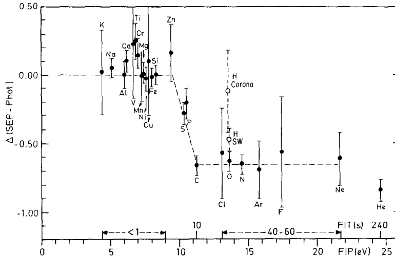
FIG. 3. Abundances of solar energetic particles (SEP) relative to the solar photosphere (Table 4). Elements K to Zn, of first ionization potential (FIP) < 10 eV, are present in normal abundance relative to Si, but elements C to Ne, of higher FIP, are depleted by an approximately constant factor. Apparently these elements are depleted in the corona by a process depending on FIP (or first ionization time, FIT). The points for P and S would fall closer to the dashed trend line if they were referenced to meteoritic rather than photospheric abundances. As H cannot be reliably determined in SEP, we plotted representative spectroscopic and solar-wind data from Table 4.
