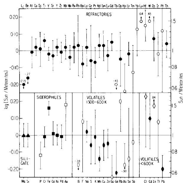
FIG. 4. Solar photospheric and meteoritic abundances (Table 2) agree rather well, except for elements affected by thermonuclear reactions (Li, Be), elements poorly determined in the photosphere (uncertain abundances or errors, or large errors: open symbols), and five problematic cases: W, Fe, Mn, Ge, and Pb (see text). If these elements are omitted, there is no systematic difference between photospheric and C1 chondrite abundances of the five major cosmochemical groups.
