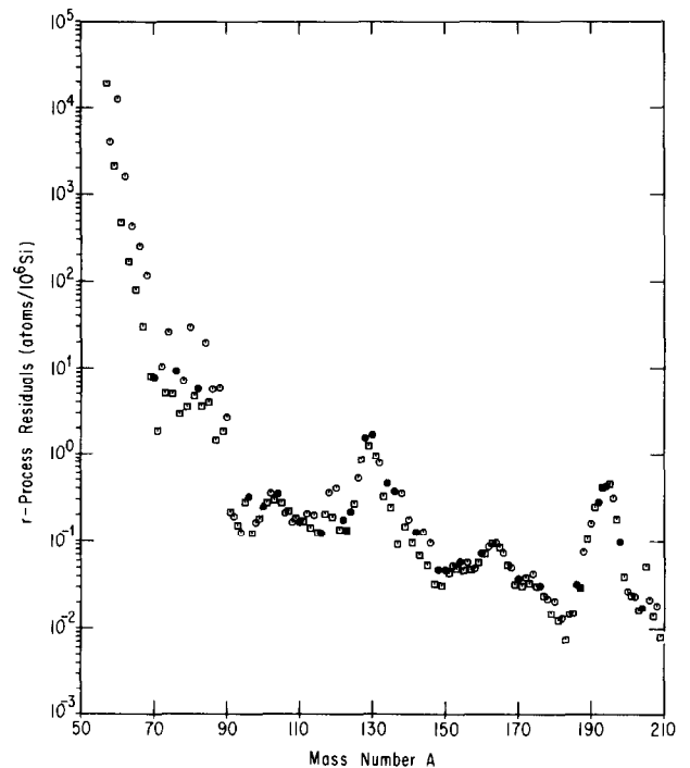
FIG. 8. (BEER, 1988, priv. commun.). To obtain the r -process component of nuclides of mixed parentage, the s -process component from Fig. 7 is subtracted from the total abundances. These “ r -process residuals” (open symbols) form a smooth curve passing through the “ r -only” nuclides (filled symbols), suggesting that the input data (abundances and cross sections) are reasonably accurate. The peaks at A \approx 130 and \approx 195 represent the enhanced abundances of short-lived, neutron-rich progenitors with closed, 82- or 126-neutron shells.
