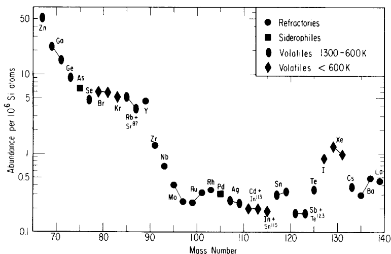
FIG. 5. Abundances of odd-mass nuclides from Zn to La are a smooth function of mass number, with elemental abundances conforming to the trend set by the isotopic ratios (tie lines). Peaks at Y, Sn, and Te-Ce correspond to closed neutron or proton shells of the nuclides themselves or their neutron-rich, shortlived progenitors in the r -process. There is no evidence for fractionation of cosmochemical groups from each other, as there are no distinct offsets at junctions where cosmochemical character changes (Ge-As-Se or Rh-Pd-Ag). The only exception is a 7% offset between Ag and Cd.
