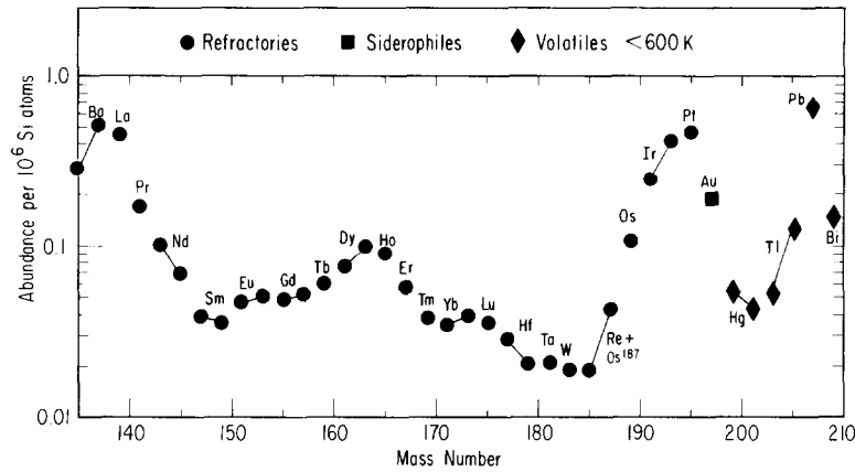
FIG. 6. The trend from Ba to Bi is likewise smooth, except that Sm is too low relative to Nd and Eu. As analytical and cosmochemical causes are ruled out (see text), it appears that the abundance curve is smooth only down to the \sim 20\% level.
