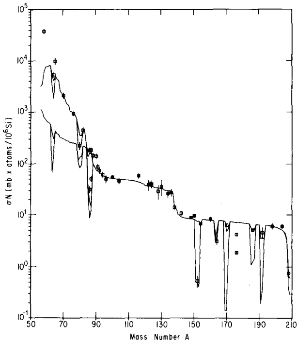
FIG. 7. (BEER, 1988, priv. commun.). In the s -process, abundance N and neutron capture cross-section \sigma are inversely proportional to each other and thus a plot of \sigma N for s -process nuclides is a function mainly of neutron exposure (KÄPPELER et al. , 1982). A computer fit to the s -only points (filled symbols) accounts for the region 90–205, but underproduces \text{Pb}^{208} and light nuclides of A < 90 . Two additional s -processes, at higher and lower fluences, are needed to account for these two regions. See text for additional discussion.
