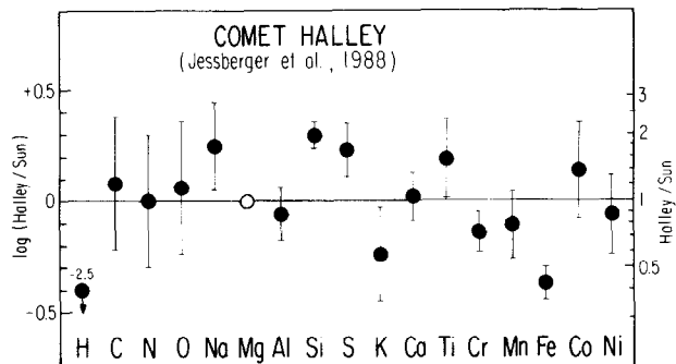
FIG. 9. Mg-normalized abundances in Comet Halley (JESSBERGER et al. , 1988) generally match those in the solar photosphere, and—for the gas/dust ratio assumed (DELSEMME, 1988)—show no deficiency for C, N, and O. However, Fe and Si are distinctly anomalous. If these values are correct, then Halley has the lowest Fe/Si ratio of any known solar-system object, except for the Moon, and cannot be pristine interstellar matter.
