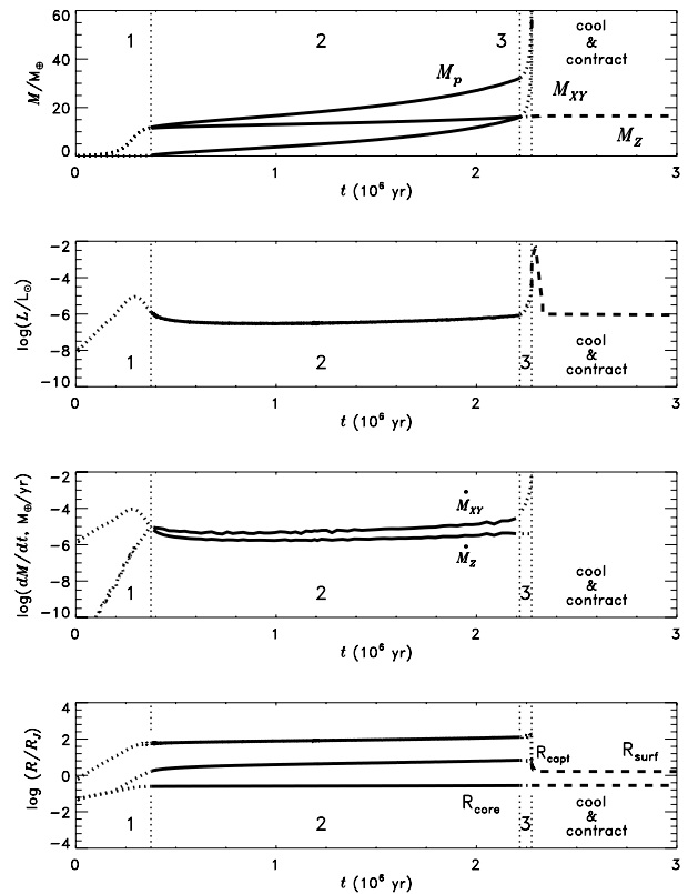
Fig. 1. The mass (units of M_{\oplus} ), the luminosity (units of L_{\odot} ), the accretion rates (units of M_{\oplus}/\text{year} ), and the radii (units of R_{\text{J}} ) are plotted as a function of time (units of million years) for the Hubickyj et al. (2005) baseline formation model of a 1 M_{\text{J}} planet. The first three phases of formation of the protoplanet (see text) are labeled. Dotted line : phase 1, solid line : phase 2, second dotted line : phase 3. The dashed line is contraction and cooling (and is merely illustrative here), at which time we switch to an evolution code with fully nongray atmosphere models.
